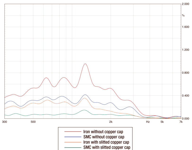
Generic example of 3rd. order distortion. This graph shows the effect on a RUBICON 8 woofer, which, with only minor details, is much alike the woofer on RUBICON 6 C.
